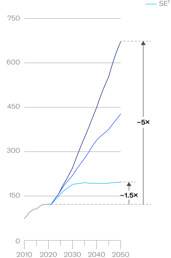
Global sustainable fuels demand outlook by scenario, Mta
