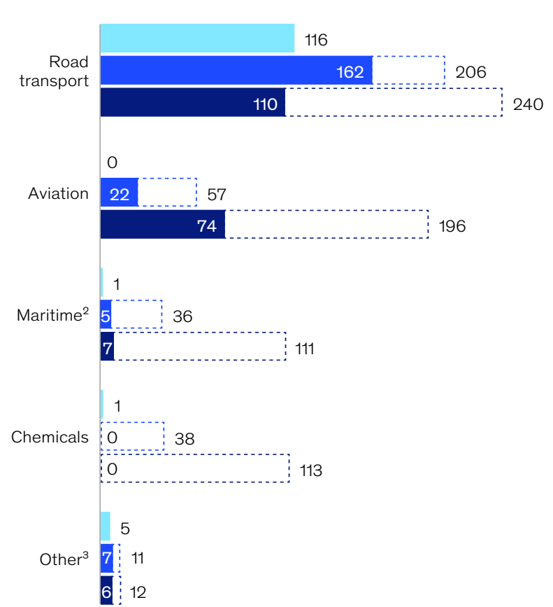
Global sustainable fuels demand by sector, SE to ST scenarios, 1 Mta
